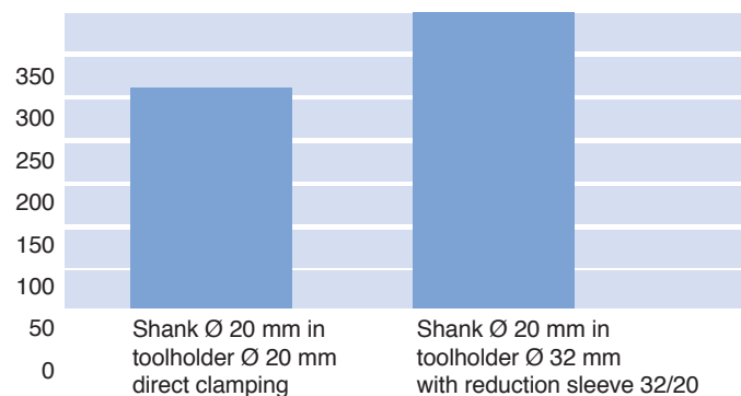
Comparison of Transmittable Torque at Ø 20 mm
