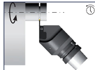
GLM 45° right hand basic tool holder + right hand cartridge
