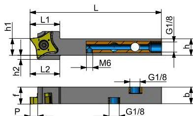
M92 QE FXCBL..HP
