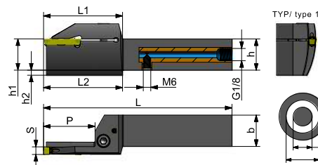
P92 1 CXCB L HP
