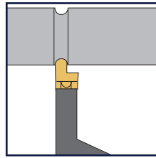
Radius profile grooving
