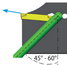
Insert in unlocked condition
