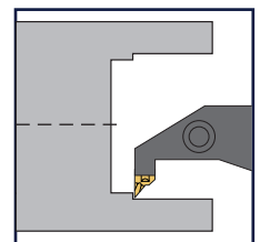
Internal profile turning
