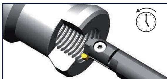
Internal threading with KOTX IR ISO ...
