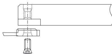
Serrage standard (A) Standard Spannsystem (A) Standard clamping system (A)
